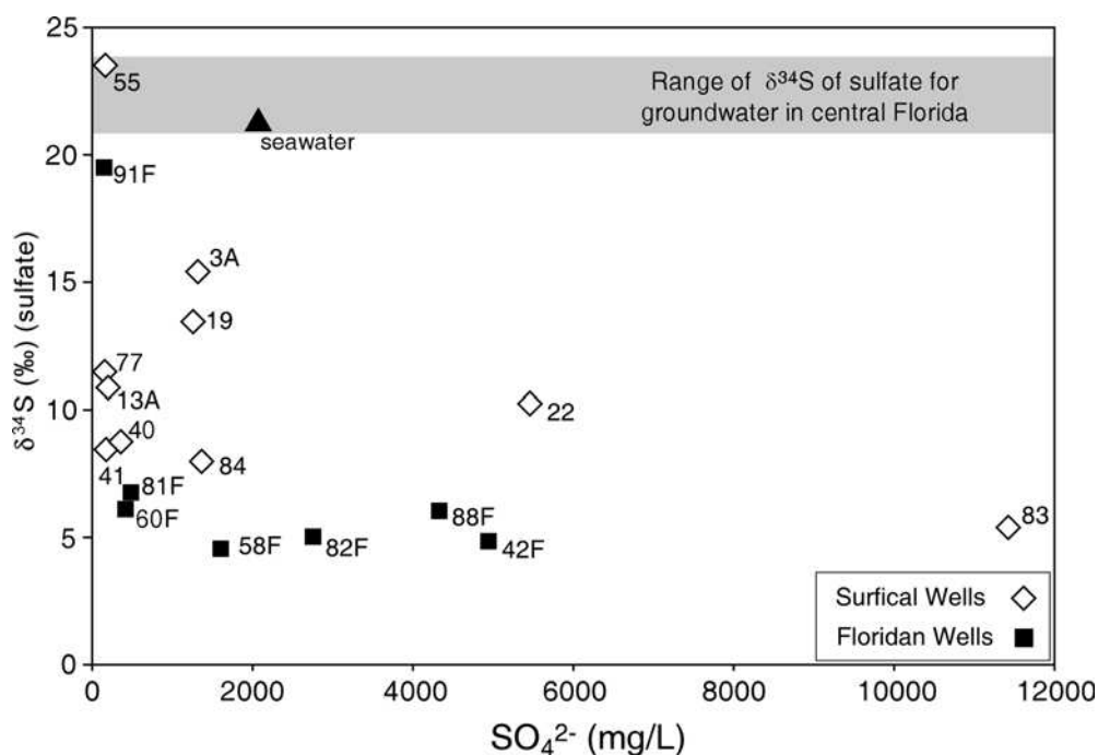
Fig. 4 \delta^{34}\text{S} in sulfate vs. concentration of \text{SO}_4^{2-} in water collected from Surficial and Upper Floridan aquifer wells. The grey area is the \delta^{34}\text{S} range for uncontaminated groundwater in central Florida from Sacks and others (1995). The \delta^{34}\text{S} value for modern seawater is from Rees and others (1978)
